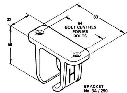
ALTERNATIVE BRACKETS
